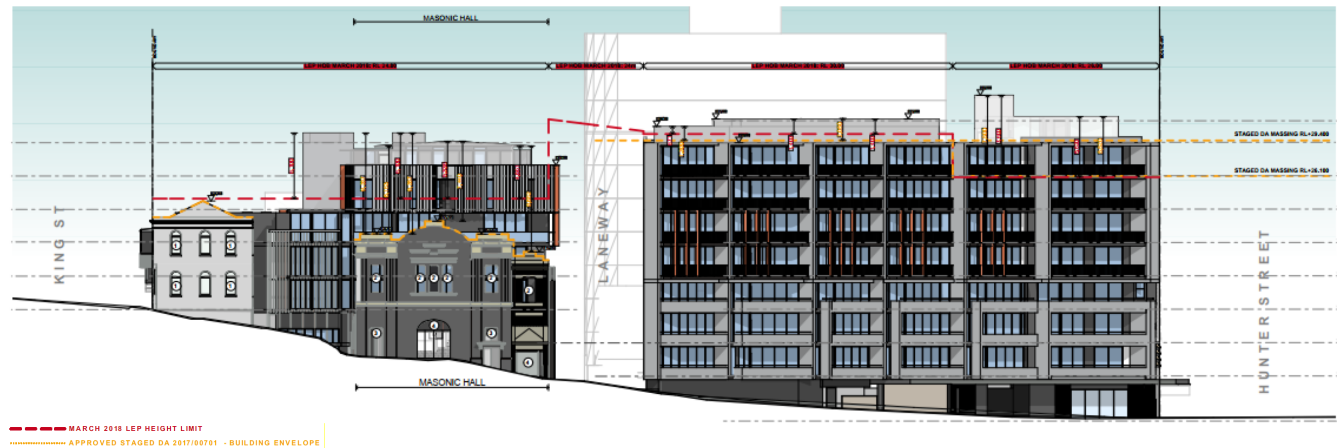
Figure 3: Variations to Height of Building Standard – Thorn Street Elevation
